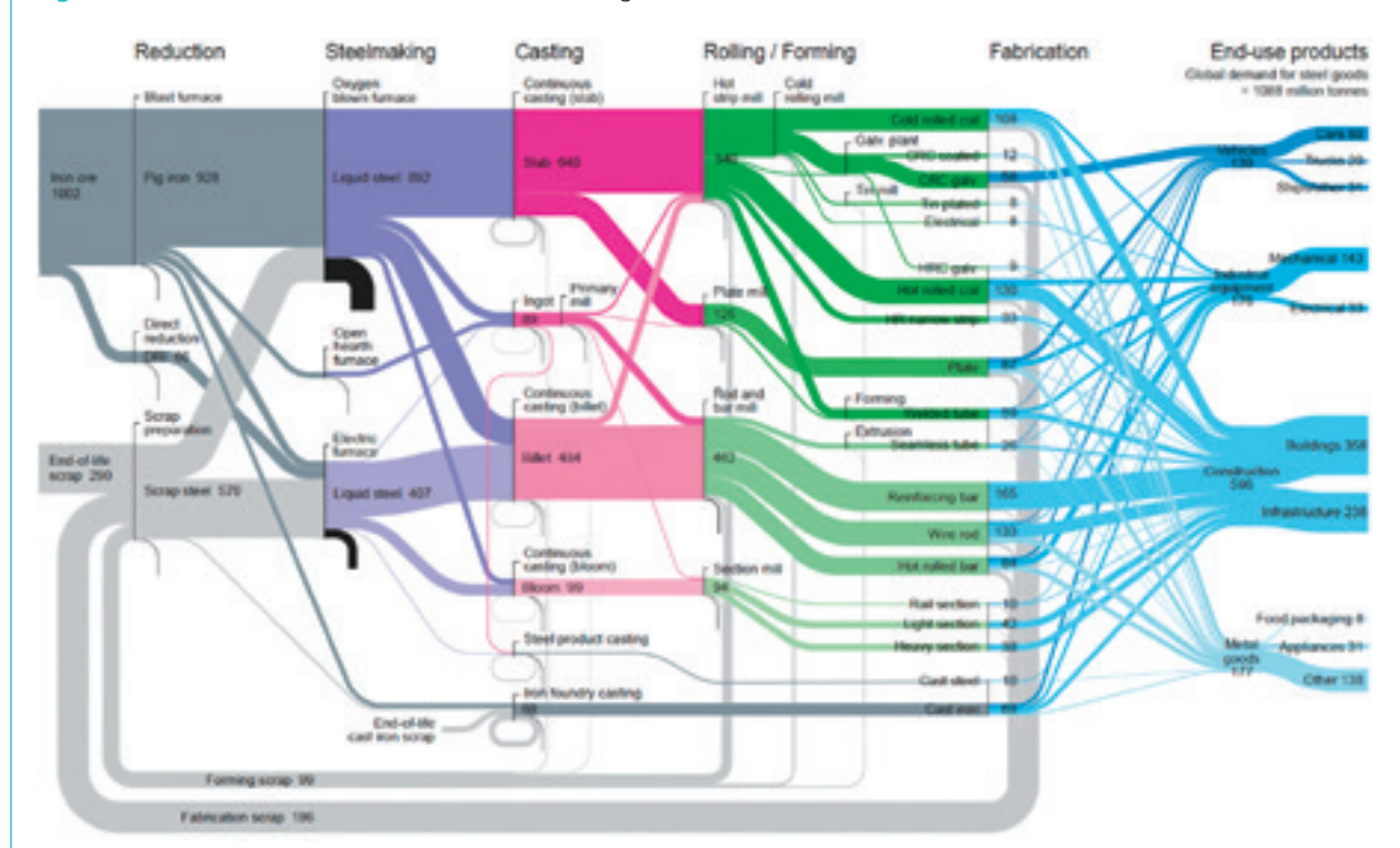
Figure 6: Global flow of steel from iron ore to end-use goods (in million tonnes, 2008) 27
